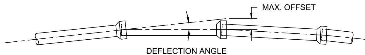
DUCTILE IRON PIPE DEFLECTION DETAIL NTS
